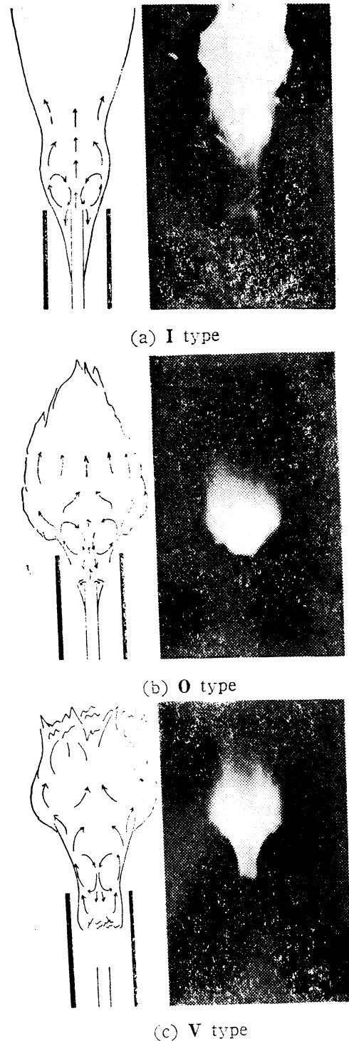
Fig. 2 Schematic diagrams and photographs of the typical flames
