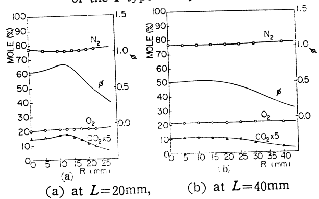
Fig. 6 Radial distributions of gas concentrations of the V type cold jet
