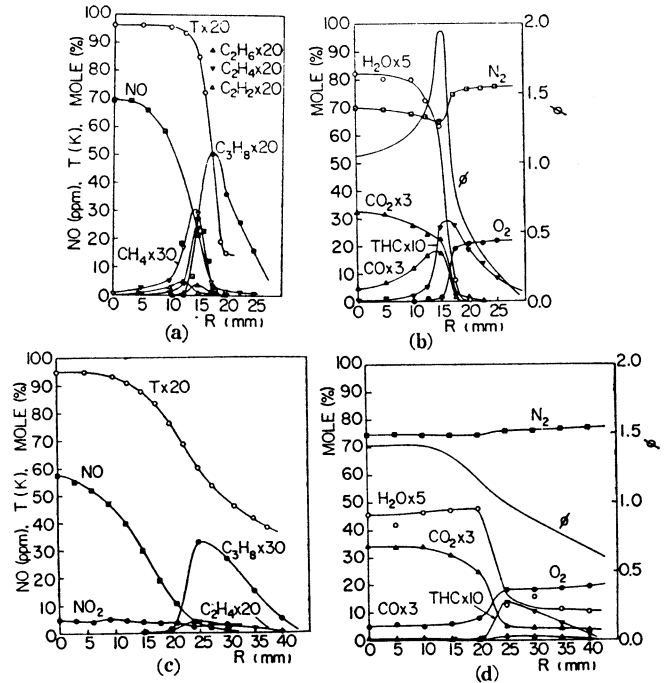
(a) Nitric oxide, hydrocarbons and temperature at L=20\text{mm} (b) Stable gases and total hydrocarbon at L=20\text{mm} (c) Nitric oxide, hydrocarbons and temperature at L=40\text{mm} (d) Stable gases and total hydrocarbon at L=40\text{mm}
