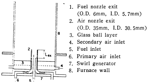
Fig. 1 Schematic diagrams of the experimental apparatus
