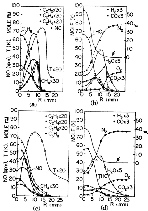
(a) Nitric oxide, hydrocarbons and temperature at L=20\text{mm} (b) Stable gases and total hydrocarbon at L=20\text{mm} (c) Nitric oxide, hydrocarbons and temperature at L=40\text{mm} (d) Stable gases and total hydrocarbon at L=40\text{mm}
